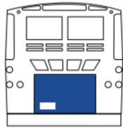
Express Tail
