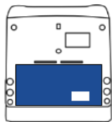
Electric Tail
