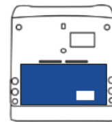
Electric Tail
